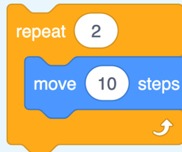
Count-controlled loop
