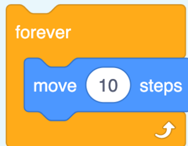
Infinite loop
